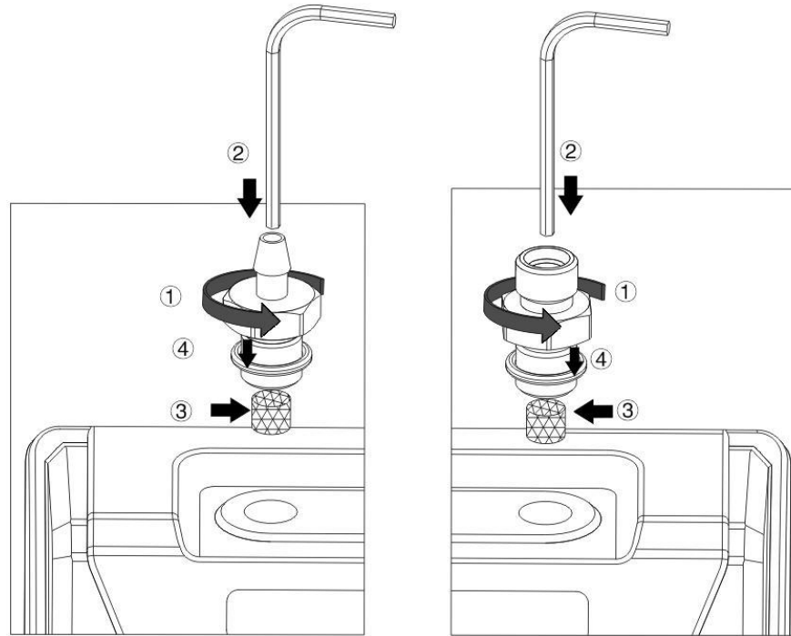
Figure 19 REF and Outlet Port Filter
