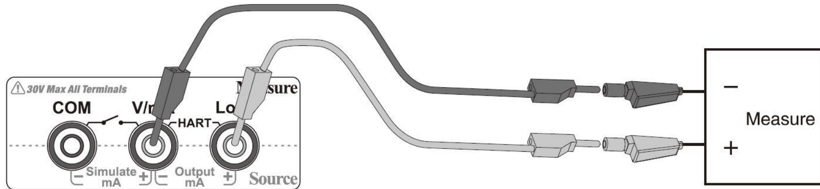
Figure 12 Current Output
