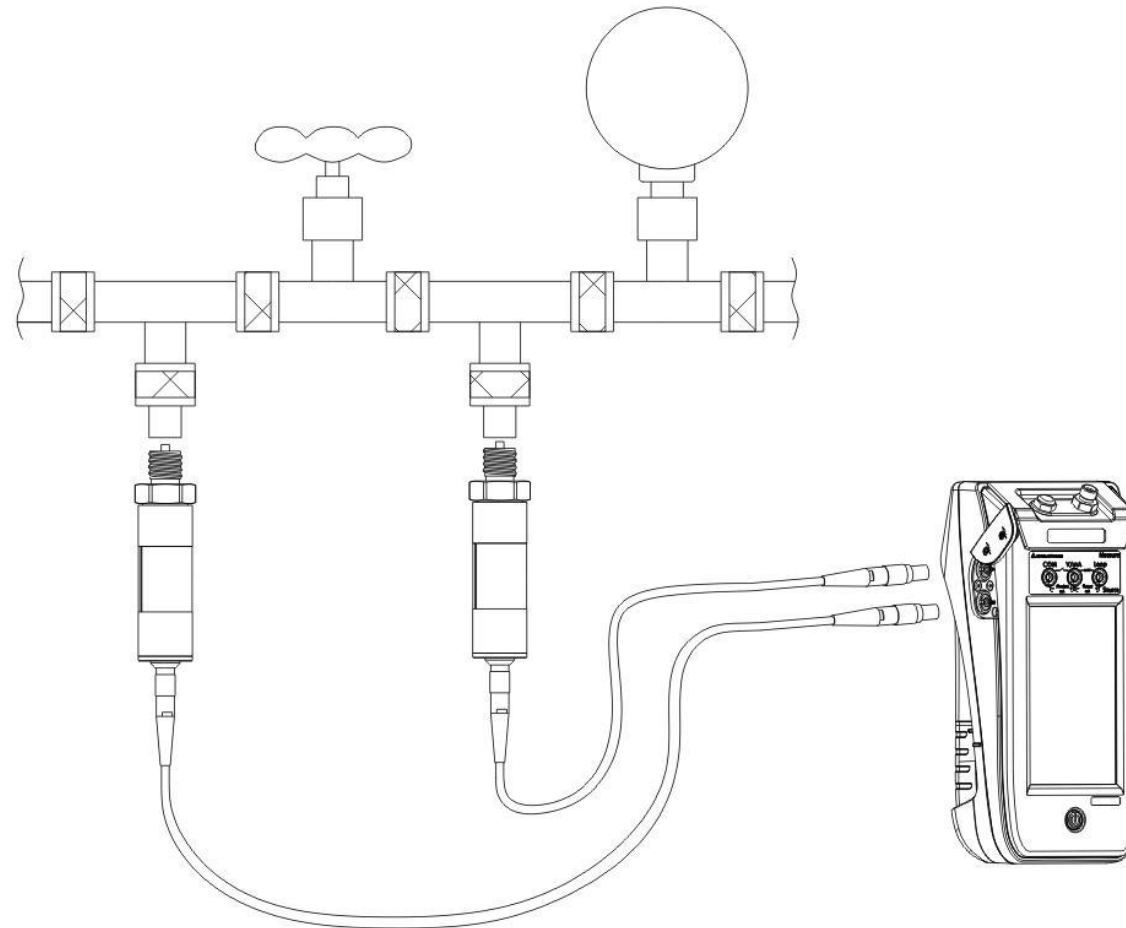
Figure 13 External Pressure Module Connection
