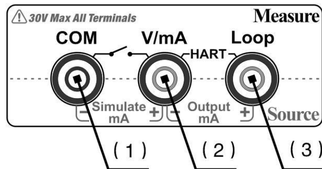
Figure 5 Electric Connection
