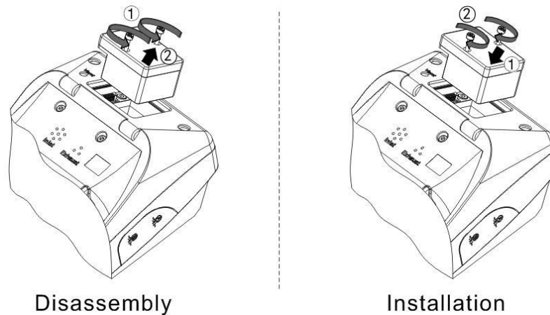
Figure 4 Internal Pressure Module Switching
