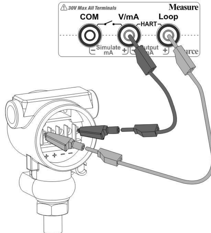
Figure 14 HART Device (Internal Power, Internal Resistor)
