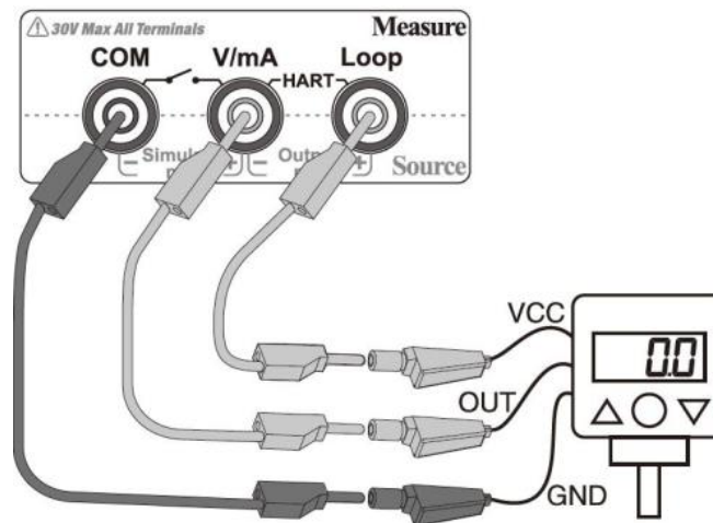
Figure 11 Electrical Switch Measurement
