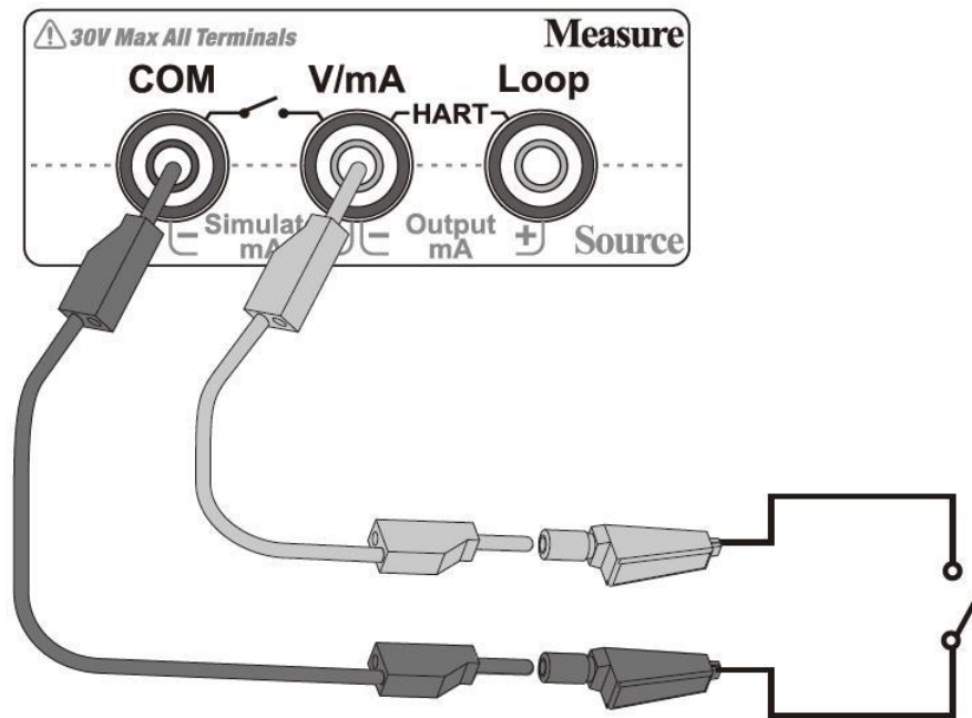
Figure 10 Mechanical Switch Measurement
