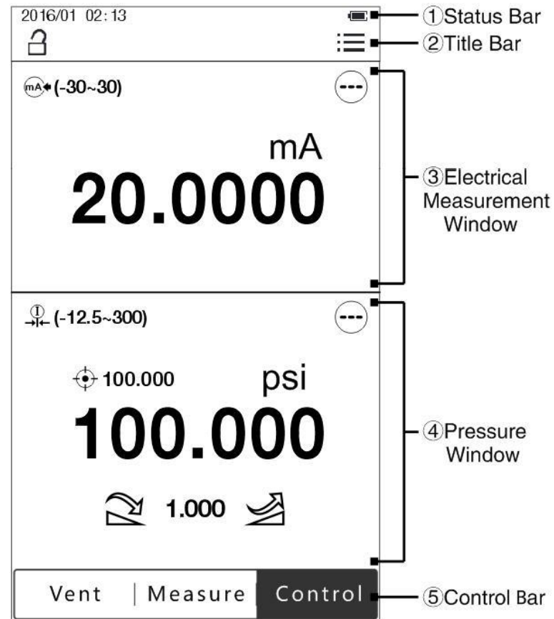
Figure 7 Main Screen
