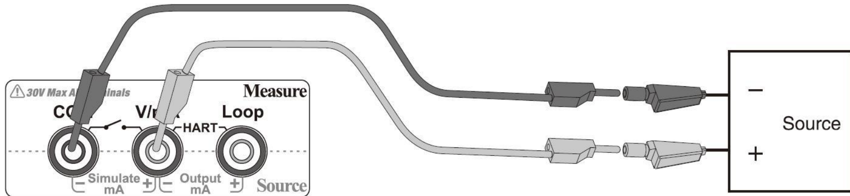
Figure 9 Current / Voltage Measurement
