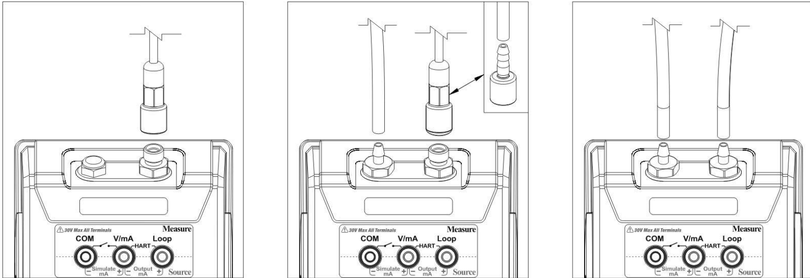
Figure 6 Pressure Connection
