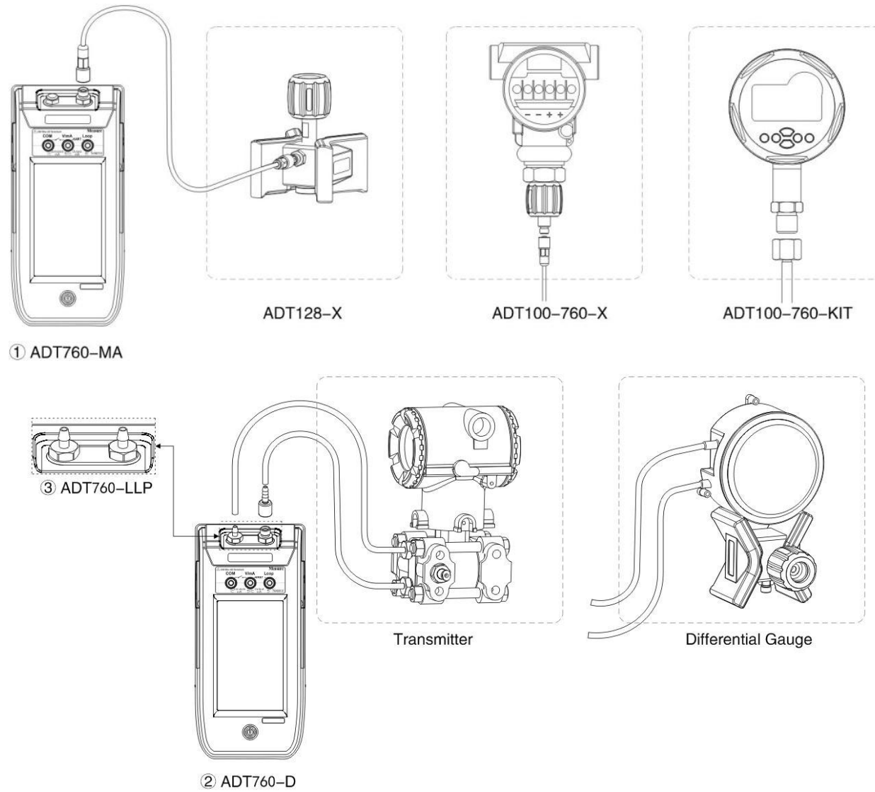
Figure 8 Output Connection
