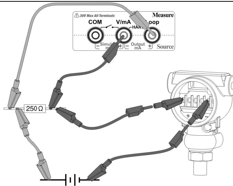
Figure 15 HART Device (External Power, External Resistor)
